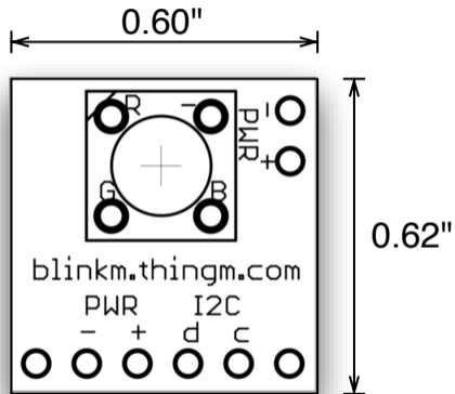
Figure 8: Packaging Information
